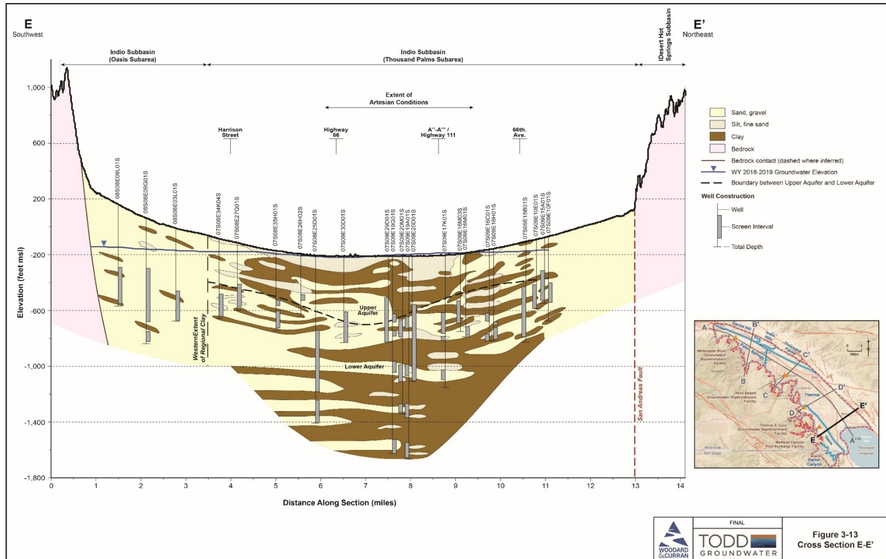
Figure 3-13. Cross Section E to E'
