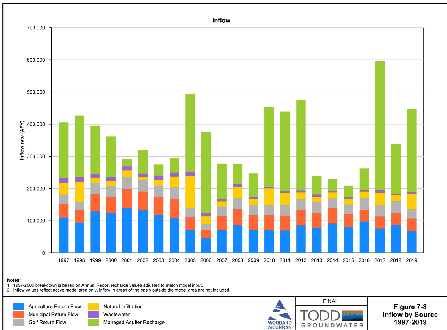
Figure 7-8. Inflow by Source 1997-2019
