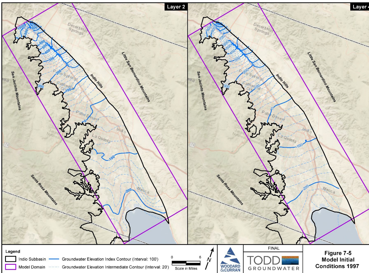
Figure 7-5. Model Initial Conditions 1997
