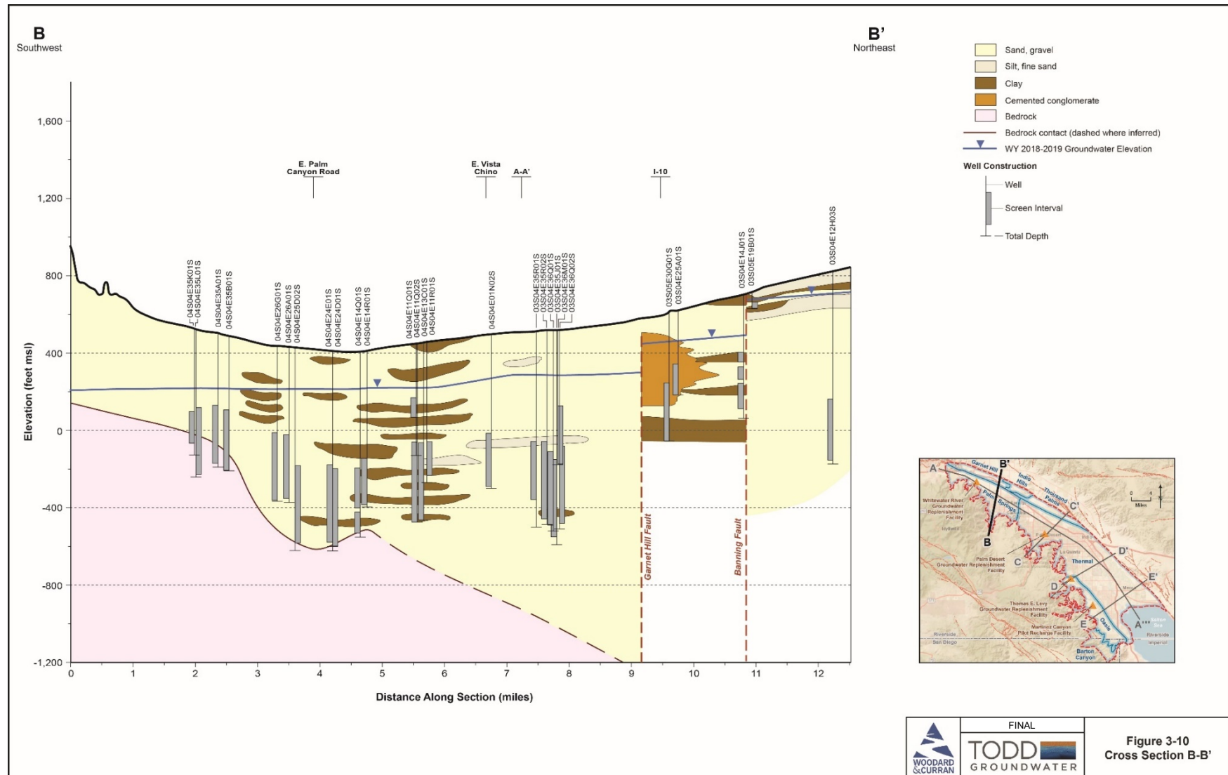
Figure 3-10. Cross Section B to B'
