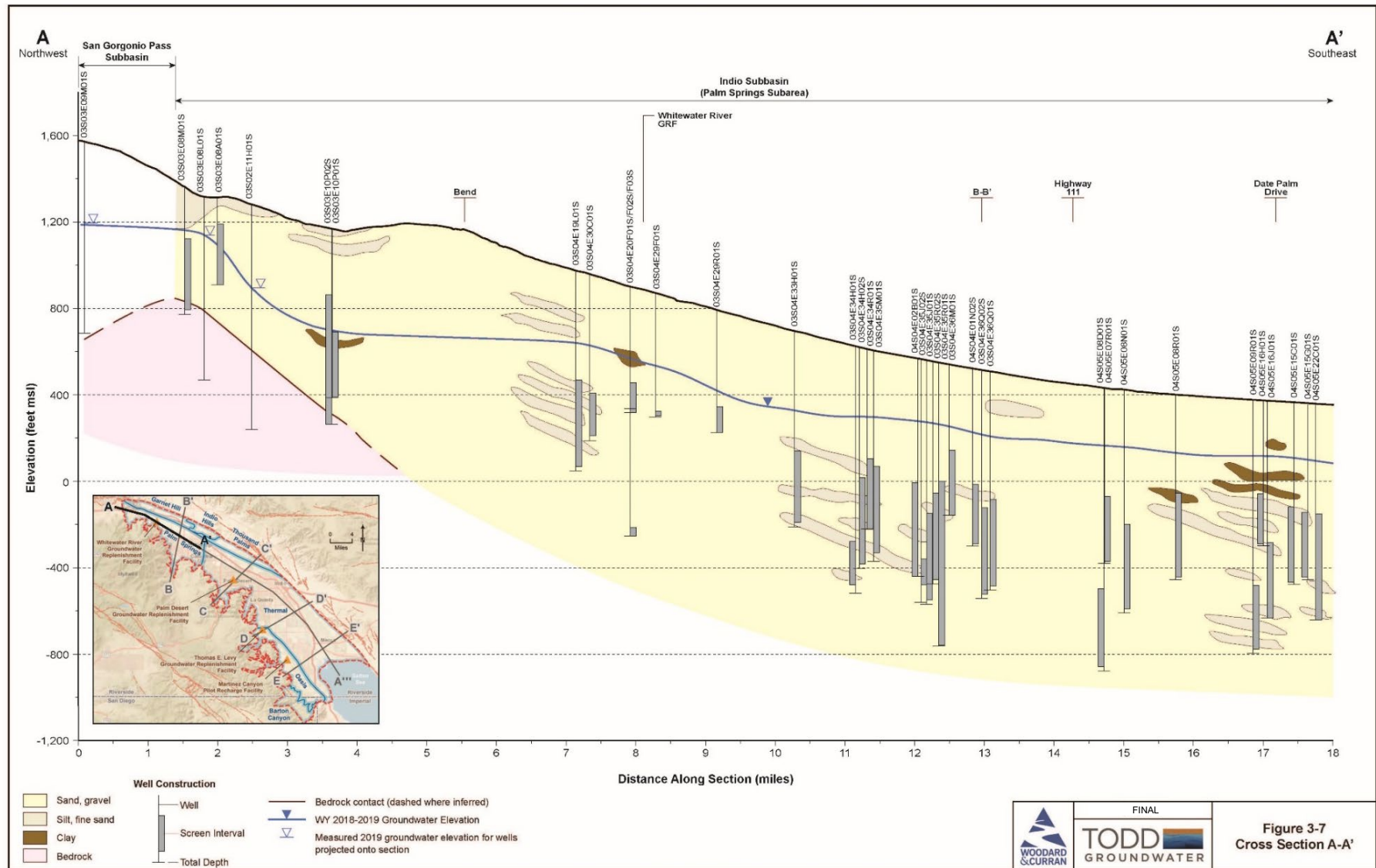
Figure 3-7. Cross Section A to A'
